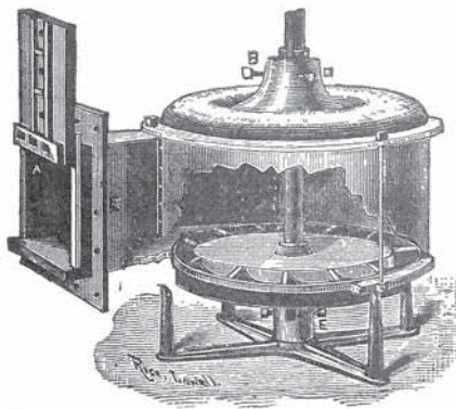
No. 2 Test Turbine.
