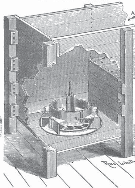
No. 1 Test Turbine.
